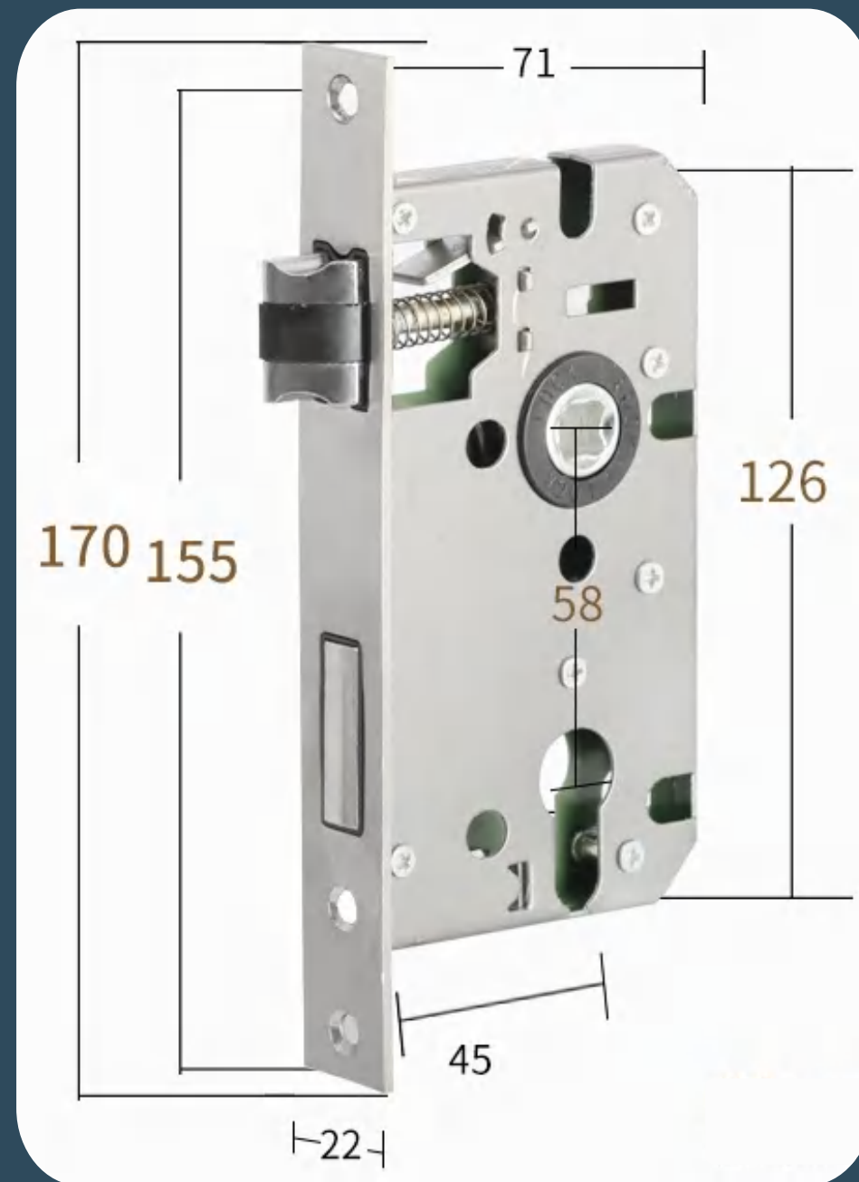
CSA5845 Basic version lock body
