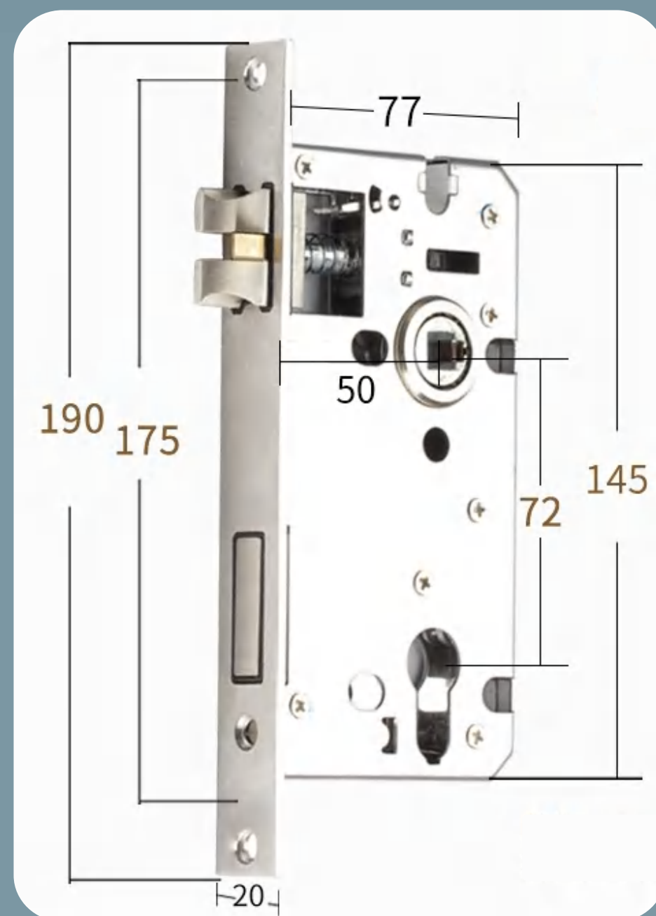
CSA7250 Steel three-prong lock body
