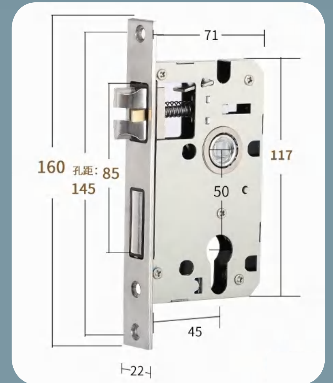
CSA5045 Steel three-prong lock body
